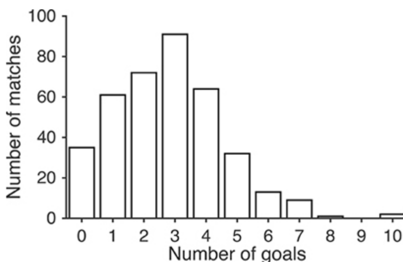
Figure 1.1 Histogram of number of goals scored during the English Premier League season 2012/13.
