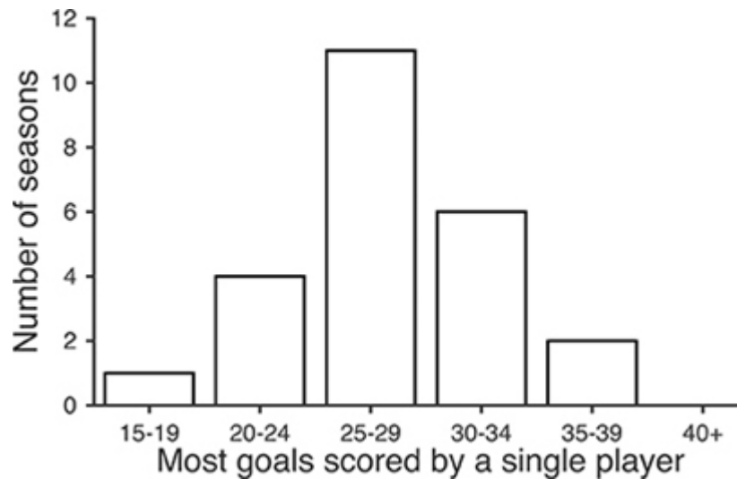
Figure 4.1 Histogram of number of goals scored by the winners of the Pichichi Trophy (for most goals scored in La Liga, Spain) between the 1986/87 and 2009/10 seasons.
