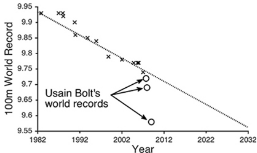
Figure 4.5 World record times for the men's 100m from 1982 to 2015. Crosses are world record times. The dots are the fitted trend line.
