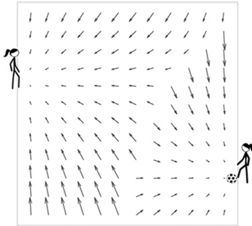
Figure 3.2 How the defender in piggy-in-the-middle should move dependent on her current position. The arrows show, for each position in the square, the direction of movement of the defender.
