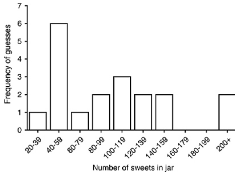
Figure 11.1 Histogram of guesses by my students of the number of sweets in a jar.
