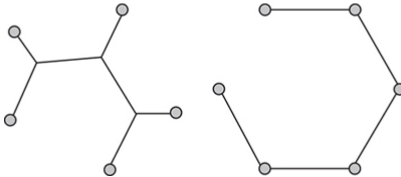
Figure N.1 Optimal solution to the problem of connecting up five suburbs on a pentagon (left) and six suburbs on a hexagon (right) using the least possible track.
