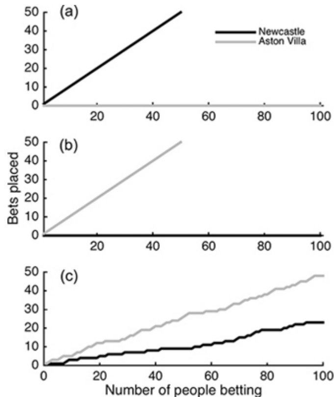
Figure 11.6 Simulation of the model where individuals use the decisions of others to make up their own mind which team they think will win the cup. Three simulations are run for the same parameter values. In the first, both the first two punters choose Newcastle (a – occurs in 49.0% of simulations). In the second simulation both the first two punters choose Aston Villa (b – occurs in 9% of simulations). In the third simulation one punter chooses Villa, the other Newcastle (c – occurs in 35.5% of simulations).
