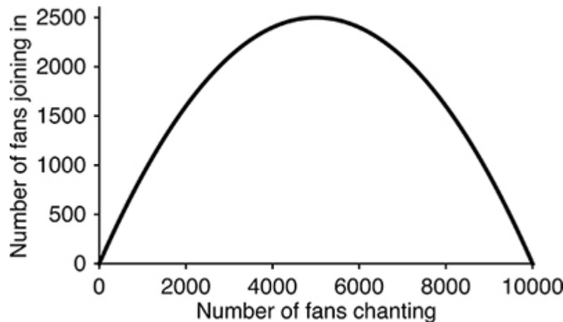
Figure N.2 Rate of increase of chanting as a function of those already chanting for logistic growth.
