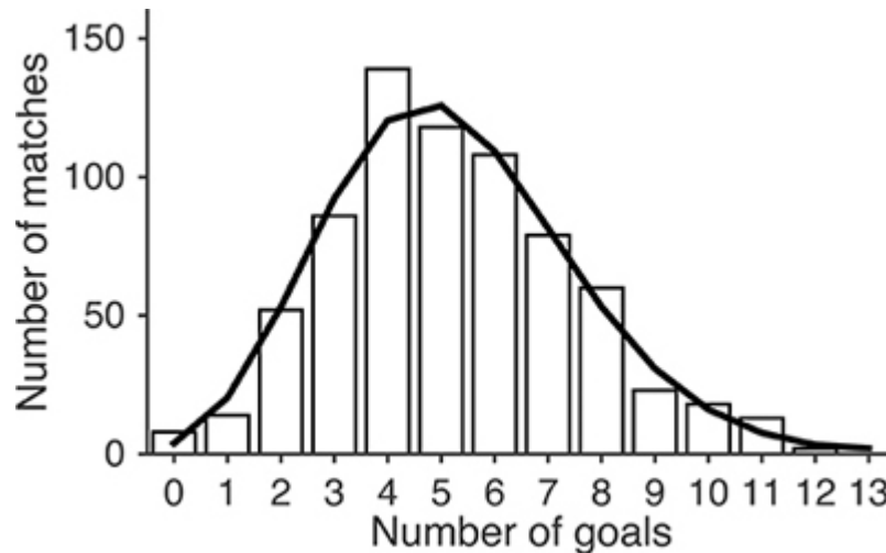
Figure 1.3 Histogram of number of goals scored during the NHL ice hockey in season 2012/13 (boxes) compared to the Poisson distribution (solid line).
