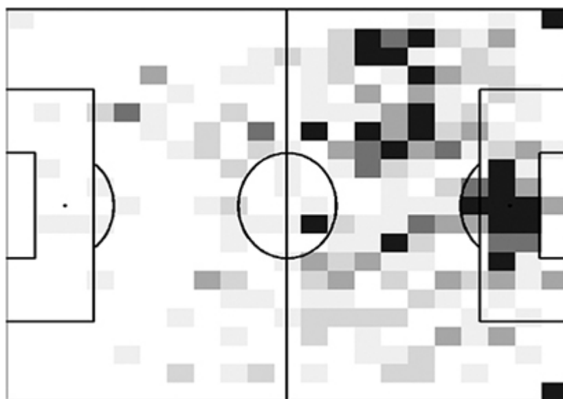
Figure 7.12 Real Madrid danger-zones during the Champions League season 2014/15. The shading is proportionally darker in areas where the ball was located during the 15 seconds leading up to a shot from the 20m by 20m area in front of the opposition goal. Data provided by Opta.
