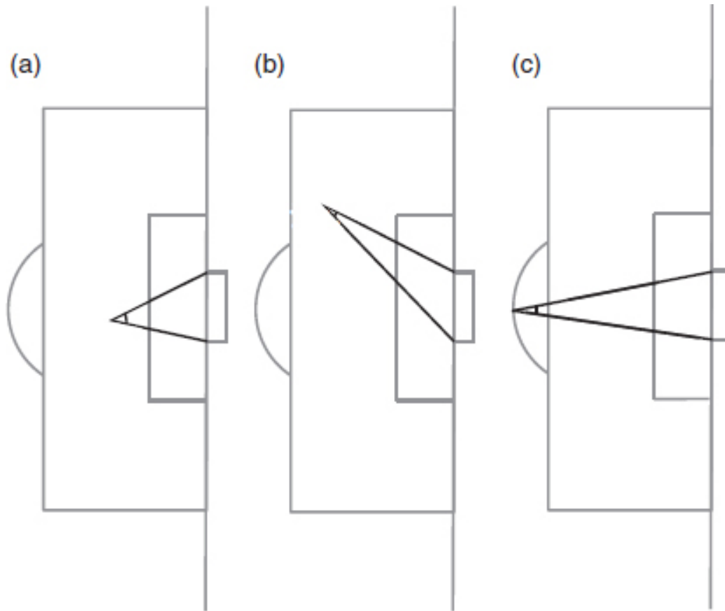
Figure 15.4 How between-post angle depend on shot position. (a) A shot close to the goal has a large between-post angle, in this case 38^\circ . Shots from a less central position (b) or further out (c) have smaller between-post angles (in both these cases the angle is 17^\circ ).
