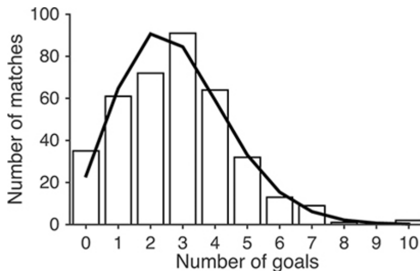
Figure 1.2 The histogram of goals during the Premier League season 2012/13 (histogram boxes) compared to the Poisson distribution (solid line).
