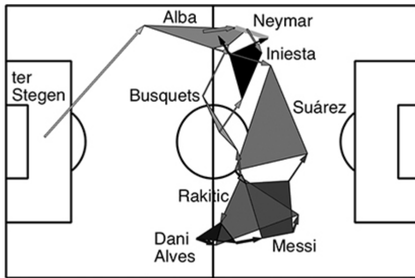
Figure 7.9 Zonal-passing network for Barcelona playing against Bayern Munich in the first leg of their Champions League semi-final in 2015. The player at the origin of each arrow passed seven or more times to the player at the tip of the arrow. The origin of the arrow is the average position from which the first player made a pass, and the tip is the average position where the second player received the pass. The thickness of the arrows is proportional to the number of passes made. The shapes associated with the players contain all the arrows in and out to that player. Data provided by Opta.
