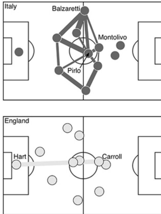
Figure 7.1 Passing networks for Italy (top) and England (bottom) in the Euro 2012 quarter-finals, showing links between pairs of players that completed 13 or more passes between them. Thicker lines indicate a higher number of passes. Both teams are attacking left to right.
