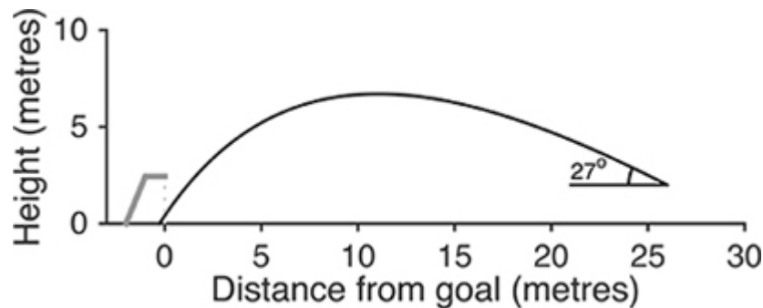
Figure 5.4 Aerodynamics of Zlatan Ibrahimovic's bicycle lob, including drag.
